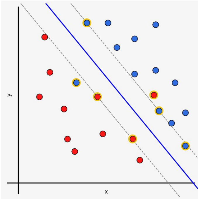
Margen suave
